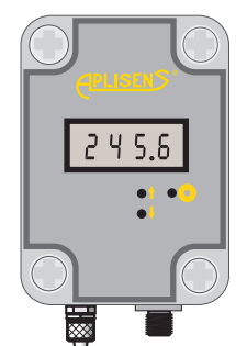
APRE-2000G/N wall-mounted version with display and local keys allowing programming, process connection PCV type. Dimensions: width: 80, height: 110, depth: 67
